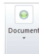
Figure 2: Document Group
