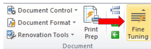
Figure 3: Fine Tuning
