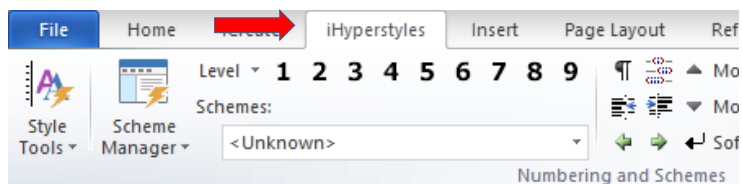
Figure 1: iHyperstyles Ribbon
